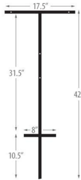
42'' T-Bar Angle Iron 3/4'' Sign Stake
